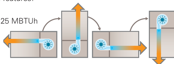
MULTI-POISE: MOST TEMPSTAR 90% GAS FURNACES CAN BE INSTALLED IN UPFLOW, DOWNFLOW, HORIZONTAL LEFT OR HORIZONTAL RIGHT CONFIGURATIONS.
